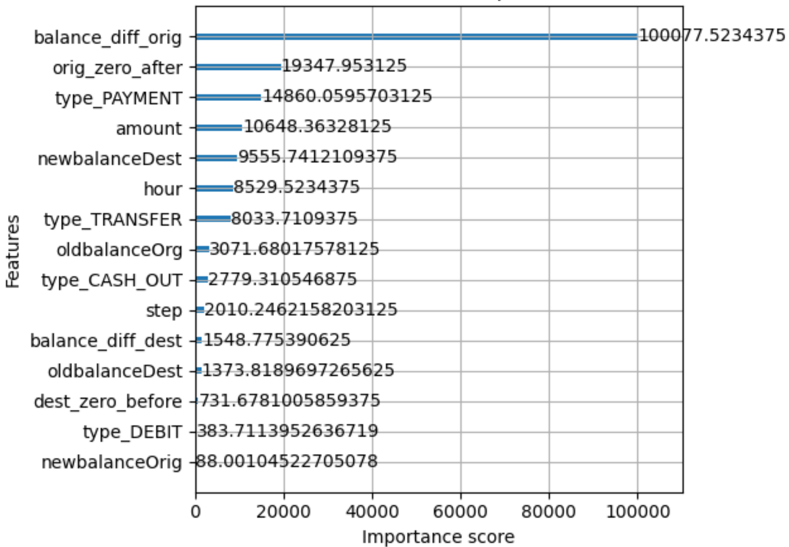
XGBoost Feature Importance
